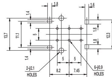
PIERCING PLAN
