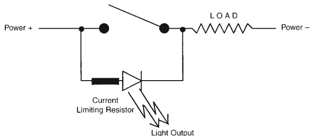
Figure 16. Wiring Diagram 1
