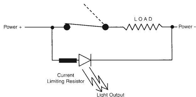
Figure 18. Wiring Diagram 3
